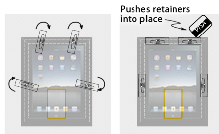
J. Finally, use a credit card to spin the frame retainers to hide them, and your frame is now locked into place! (Hint: Use a credit card to remove/dismount the frame)
