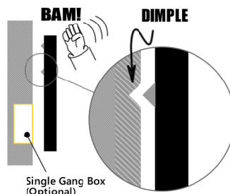
B. Position the frame and dimple the wall to mark the drill points
